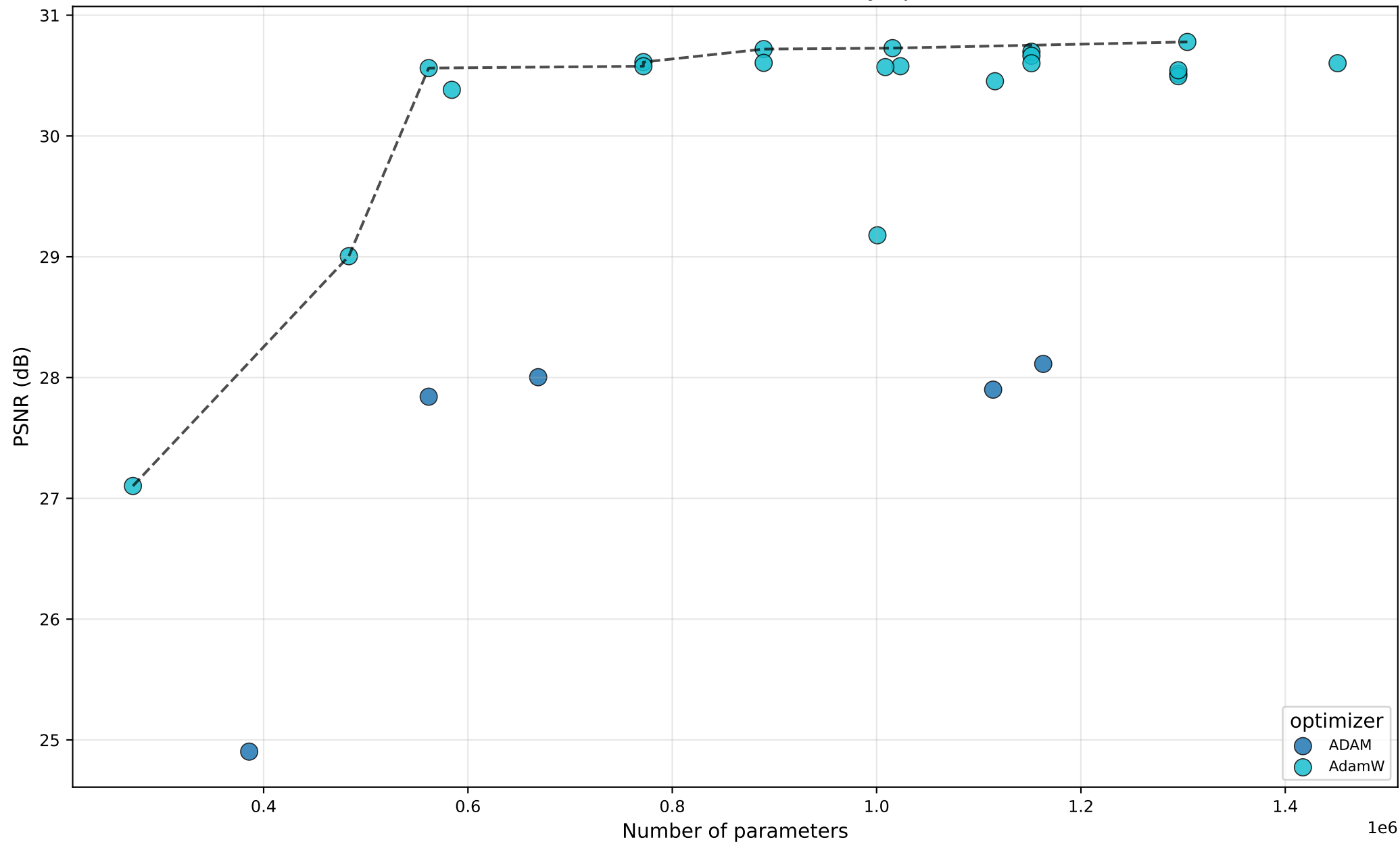
PSNR vs #Params — OmniSR — by optimizer
